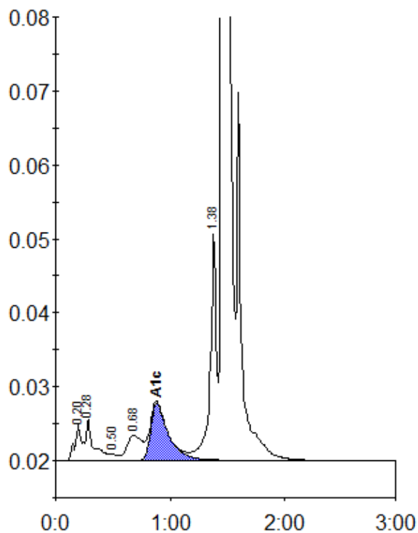
Peak table - ID: 10181986
